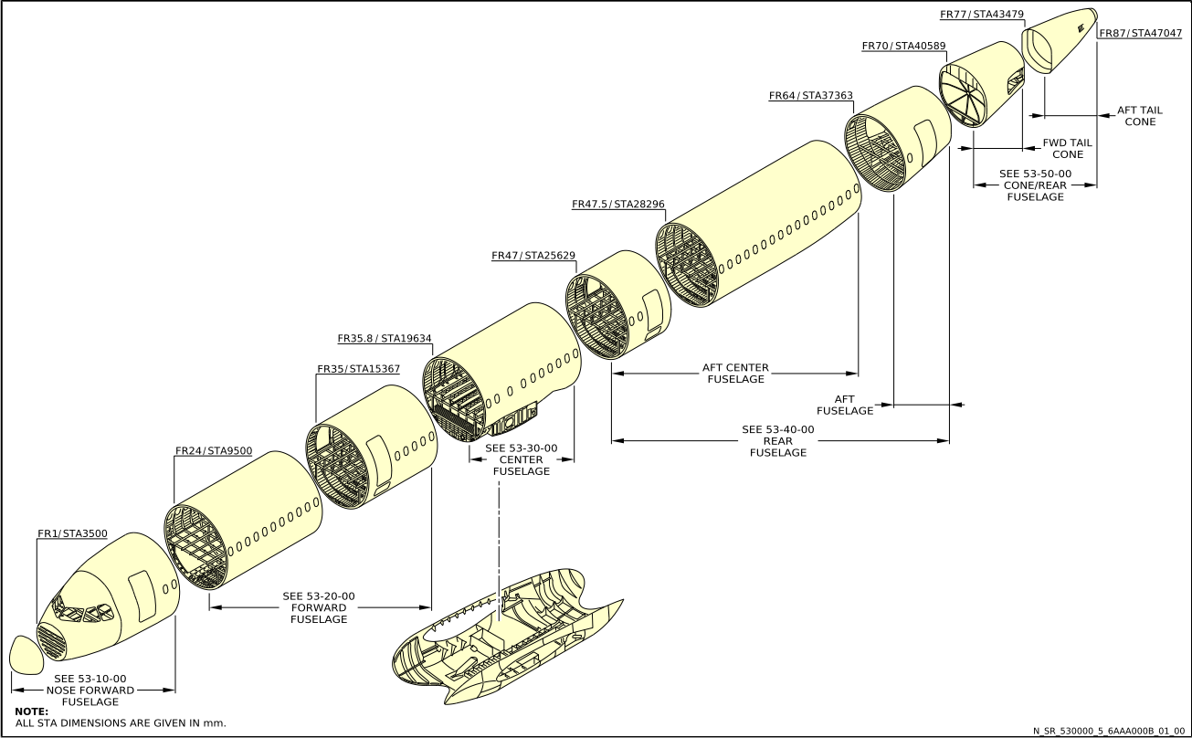
Figure 001 / 53-00-00 (SHEET 1) - Fuselage - Section Division
