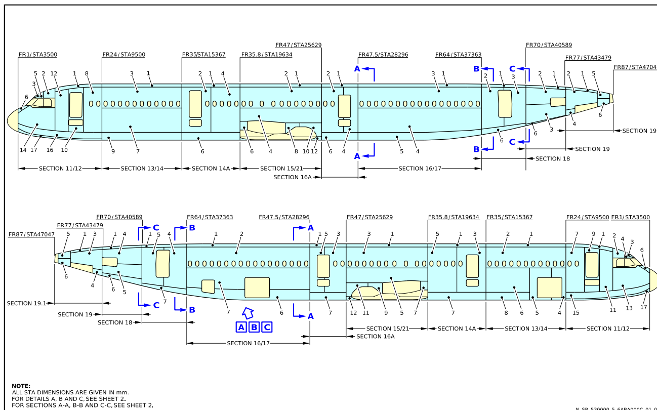
Figure 002 / 53-00-00 (SHEET 1/2) - Fuselage - Main Panel and Section Configuration
