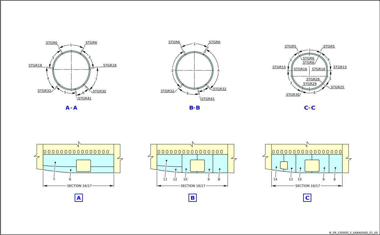
Figure 002 / 53-00-00 (SHEET 2/2) - Fuselage - Main Panel and Section Configuration
